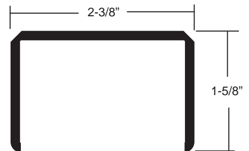
Top Rail Profile
