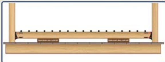
STEP #4 - Cut two (2) "Spacer Blocks" to be placed between deck & bottom rail. Place bottom rail section between posts. Install four (4) #8 x 2" screws (per connector) through railing connectors into posts
