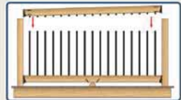
STEP #6 - Start Top Rail at an angle and insert connectors into balusters or balusters into insertion holes in top rail. Make sure balusters are fully connected. Install four (4) #8 x 2" screws (per connector) through railing connectors into posts. NOTE: With spans greater than 6' (or required), install a foot block (use cut-off from rail).
