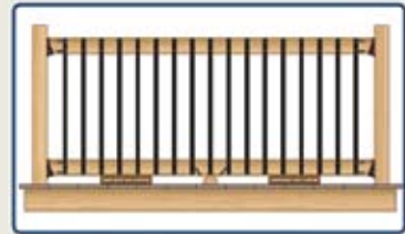
STEP #6 - Rest rail section on two (2) temporary spacer blocks the required height between deck and bottom of bottom rail. Center railing connectors on post and install four (4) #8 x 2" screws (per connector) through railing connector into posts. NOTE: With spans greater than 6' (or required), install a foot block (use cut-off from rail).
