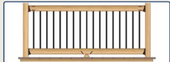
STEP #5 - Place top rail into position. Install four (4) #8 x 2" screws (per connector) through railing connectors into posts. NOTE: With spans greater than 6' (or required) install a foot block (use cut-off from rail).
