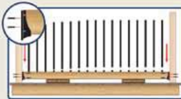
STEP #5 - Install two (2) #8 x 2" screws (per connector) through railing connector into rail ends. Rest bottom rail on two (2) temporary spacer blocks the required height between deck and bottom of bottom rail. Center railing connectors on post and install four (4) #8 x 2" screws (per connector) through railing connector into posts. Apply a small amount of silicone caulk to diameter of baluster where it meets baluster connector or insertion hole to insure a tight, movement-free installation. Install balusters on bottom rail.
