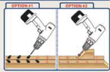
STEP #3 - There are two options for installing balusters. Option #1 - Connector Method: Insert screw through connector and install where lines intersect (start screw vertically and tilt screw to proper angle). Top and bottom baluster connectors will be facing opposite directions. Do not overtighten. Option #2 - Insert Method: Drill a 3/4" hole, 3/4" deep in top and bottom rails where lines intersect using a rail cut-off as a guide block for stair angle.
